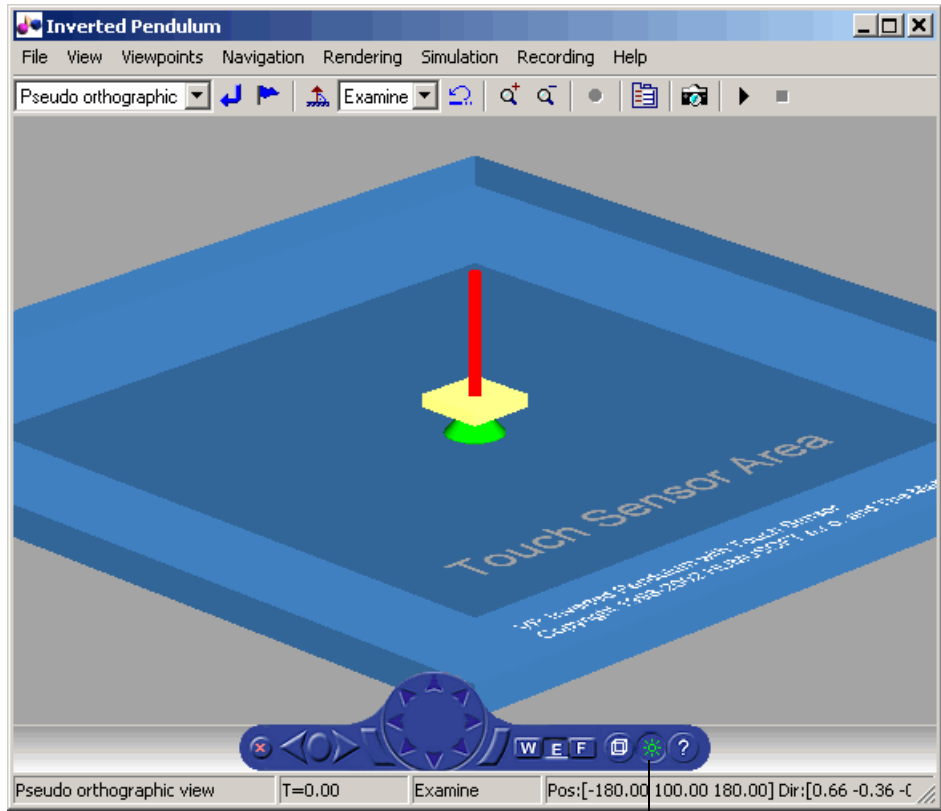
Headlight toggle
